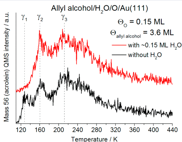
Figure 5. TPD spectra for acrolein ( m/z = 56 ) following adsorption of 3.6 ML of allyl alcohol on the Au(111) surface populated with 0.15 ML of atomic oxygen and 0.15 ML of atomic oxygen followed by \sim 0.15 ML of \text{H}_2\text{O} . All species were adsorbed at a sample temperature of 77 K.
