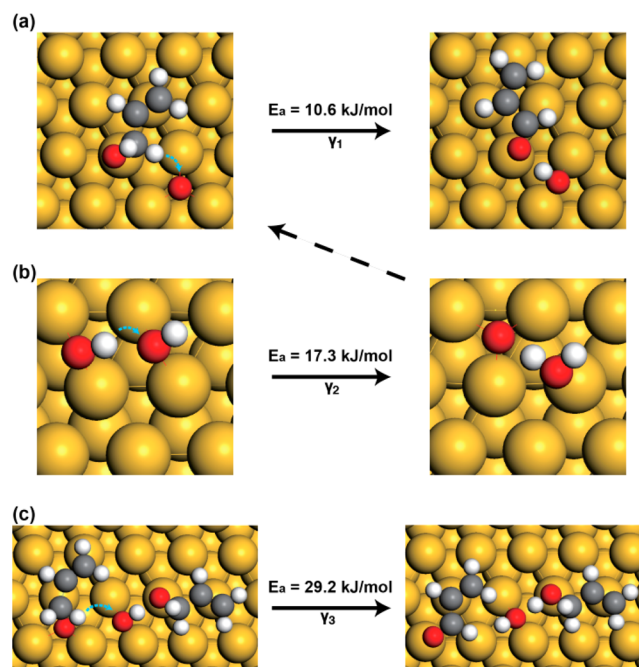
Scheme 2. Proposed Mechanistic Pathways for \alpha -Dehydrogenation of Allyloxide To Generate Acrolein on the O/Au(111) Surface a
