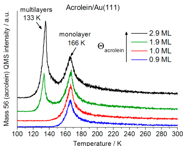
Figure 2. TPD spectra for acrolein ( m/z = 56 ) desorption from Au(111). Acrolein was adsorbed on the Au(111) surface at a sample temperature of 77 K.
