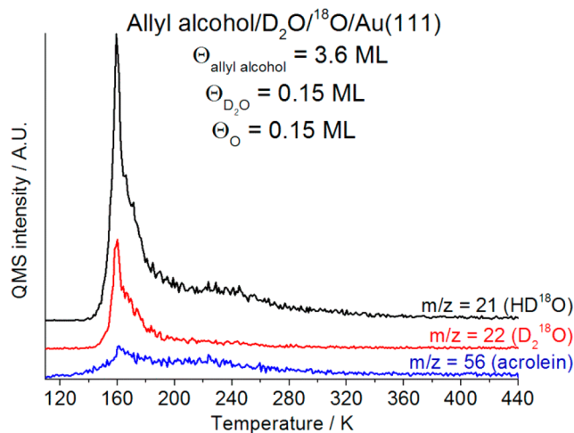
Figure 6. TPD spectra for acrolein ( m/z = 56 ), \text{HD}^{18}\text{O} ( m/z = 21 ), and \text{D}_2^{18}\text{O} ( m/z = 22 ) following adsorption of 3.6 ML of allyl alcohol on the Au(111) surface populated with 0.15 ML of ^{18}\text{O} and 0.15 ML of \text{D}_2^{16}\text{O} . All species were adsorbed at a sample temperature of 77 K.
