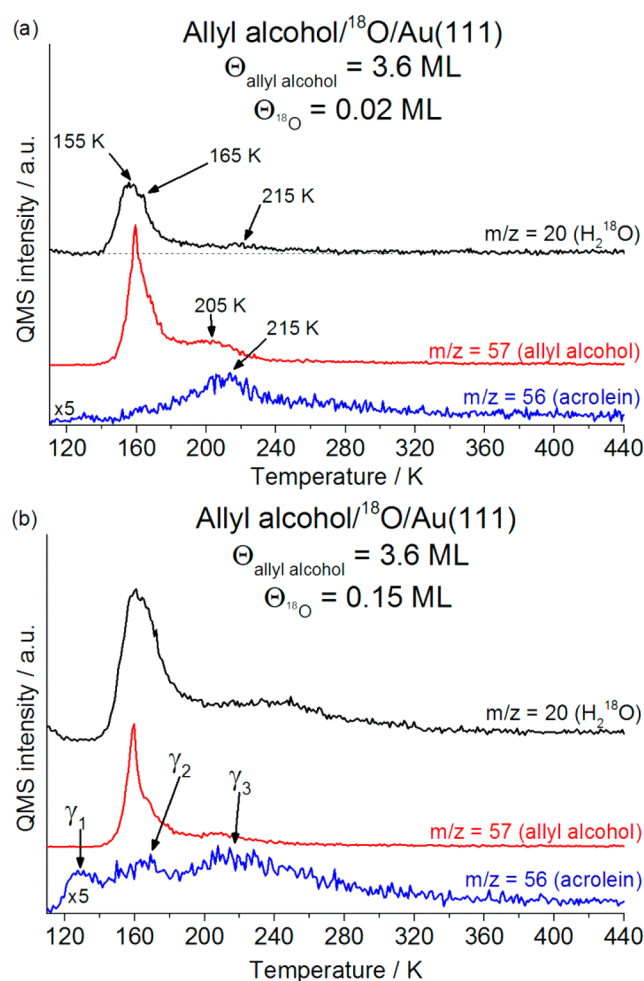
Figure 3. TPD spectra for acrolein ( m/z = 56 ), allyl alcohol ( m/z = 57 ), and \text{H}_2^{18}\text{O} ( m/z = 20 ) following adsorption of 3.6 ML of allyl alcohol on the Au(111) surface populated with (a) 0.02 ML of ^{18}\text{O} and (b) 0.15 ML of ^{18}\text{O} . Allyl alcohol and ^{18}\text{O} were adsorbed at a sample temperature of 77 K.
