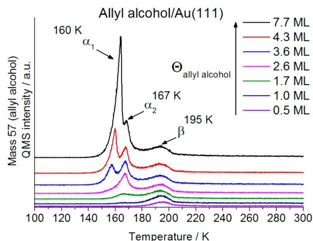
Figure 1. TPD spectra for allyl alcohol ( m/z = 57 ) desorption from \text{Au}(111) . Allyl alcohol was adsorbed on the \text{Au}(111) surface at a sample temperature of 77 K.
