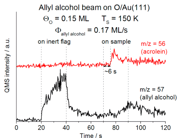
Figure 4. RMBS of allyl alcohol on 0.15 ML of O/Au(111). Allyl alcohol was dosed onto the sample at a surface temperature of 150 K while monitoring acrolein ( m/z = 56 ) production and allyl alcohol ( m/z = 57 ) desorption via QMS. Atomic oxygen was adsorbed at a sample temperature of 77 K. The flux of allyl alcohol on the surface was 0.17 ML/s.
